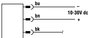
Quick-Disconnect Hookup
