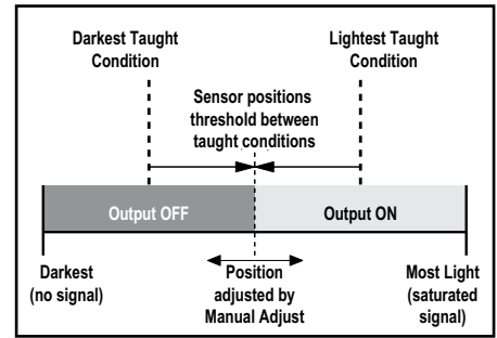
Figure 2. Two-Point Dynamic TEACH (Light Operate shown)
