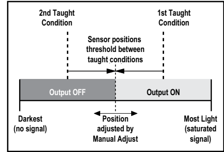
Figure 3. Two-Point TEACH (Light Operate shown)
